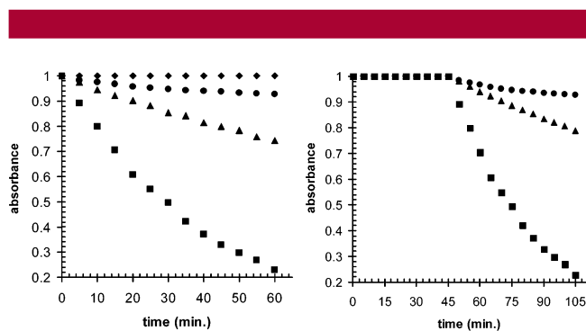
Figure 1. (A) (left) The change in the absorbance (at 415 nm) of 1,3-diphenylisobenzofuran (50 \mu M) in 2-propanol under red-light illumination in the presence of 5.0 \mu M dyes (circles, 1 ; triangles, 2 ; squares, 3 ); and diamonds, no added dye. (B) (right) Same concentration of dyes (circles, 1 ; triangles, 2 ; squares, 3 ) and DPBF; illumination starts after 45 min dark treatment.
