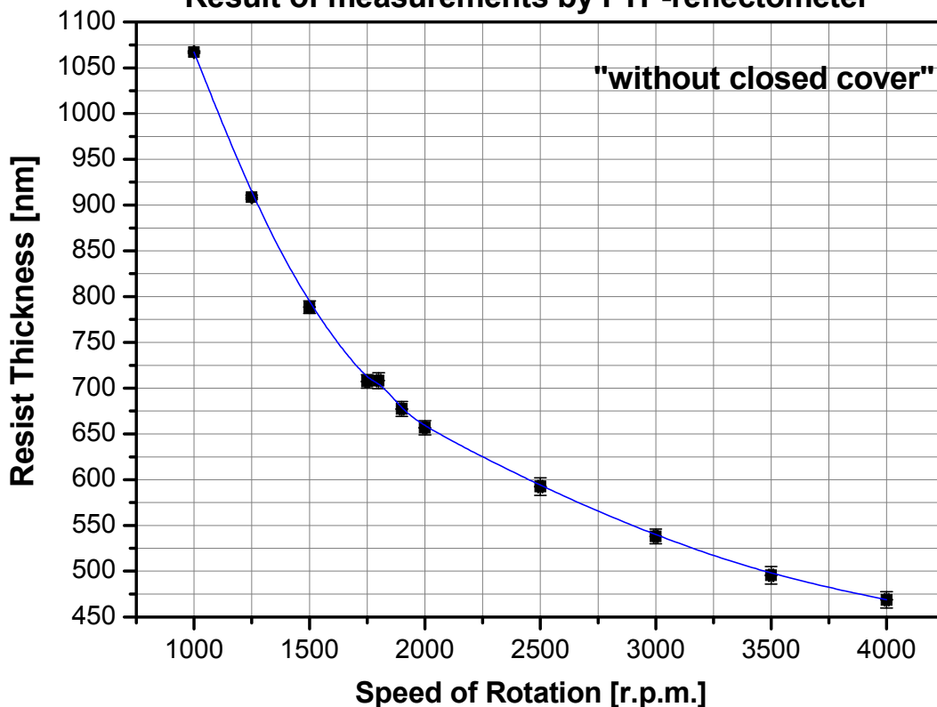
E-beam-resist NANO 950K PMMA A6, in anisol (MicroChem) Result of measurements by FTP-reflectometer
